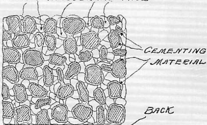
FIG. 1 INTERCOMMUNICATING CHANNELS EXTENDING TO AND OPENING THROUGH THE FACE
